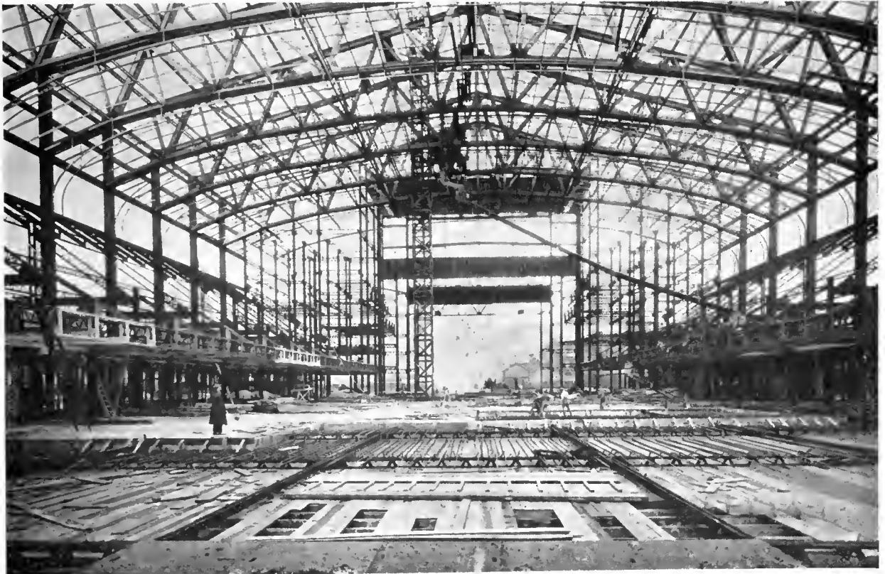
A VIEW FROM THE MAIN FLOOR DURING STEEL ERECTION
